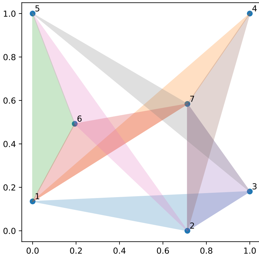
The 8 minimal area triangles for n=7
